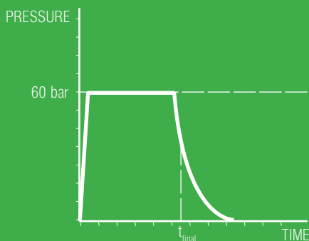
WITH CONSTANT FLOW TECHNOLOGY VALVE
