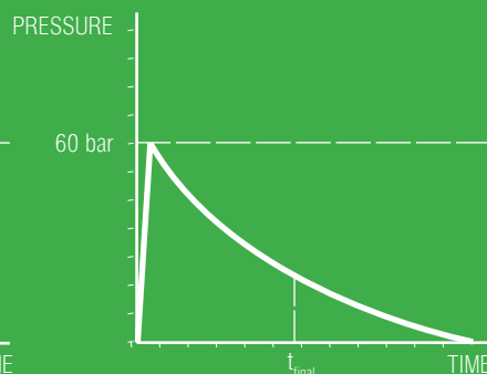
WITH STANDARD VALVE SYSTEM
