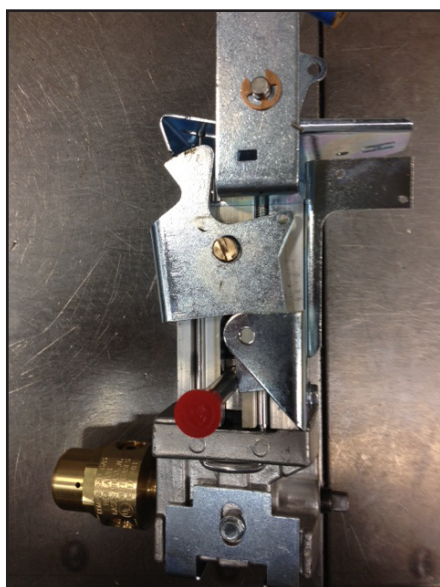
Old Release Mechanism
